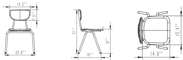
HP01-18 18" seat Height
