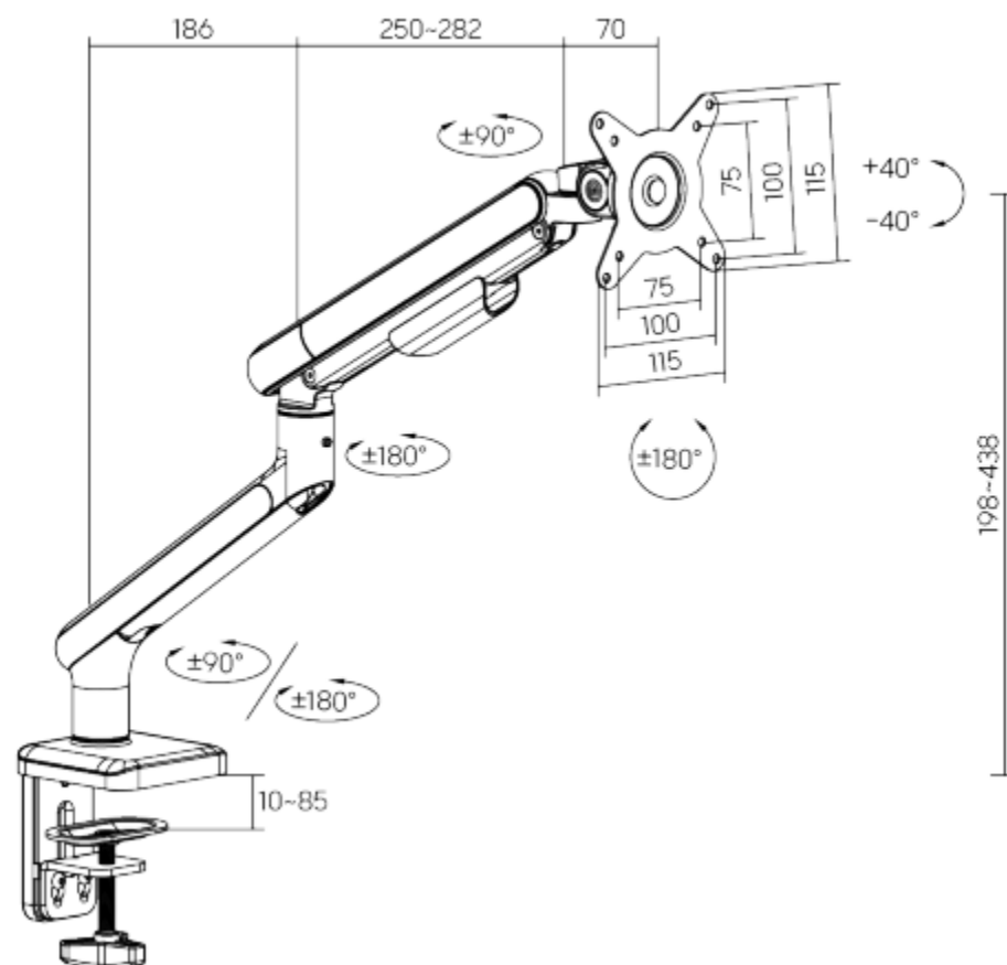
Dimensions (mm)
