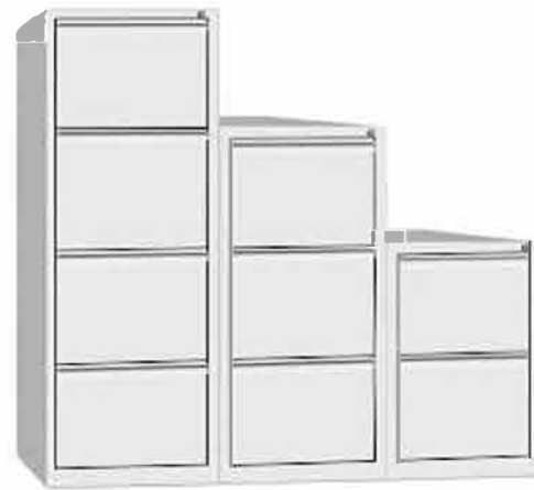
MY-FC-001-4D/3D/2D H1325/1025/725*W460*D620mm
